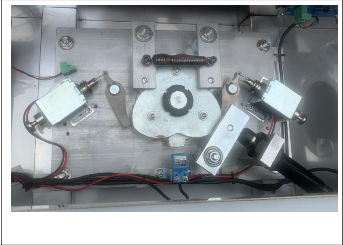
electromagnetic motor with buffer function
